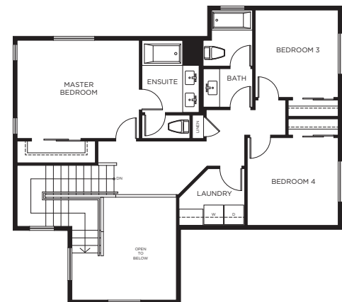
UPPER FLOOR (4 BED OPTION)
